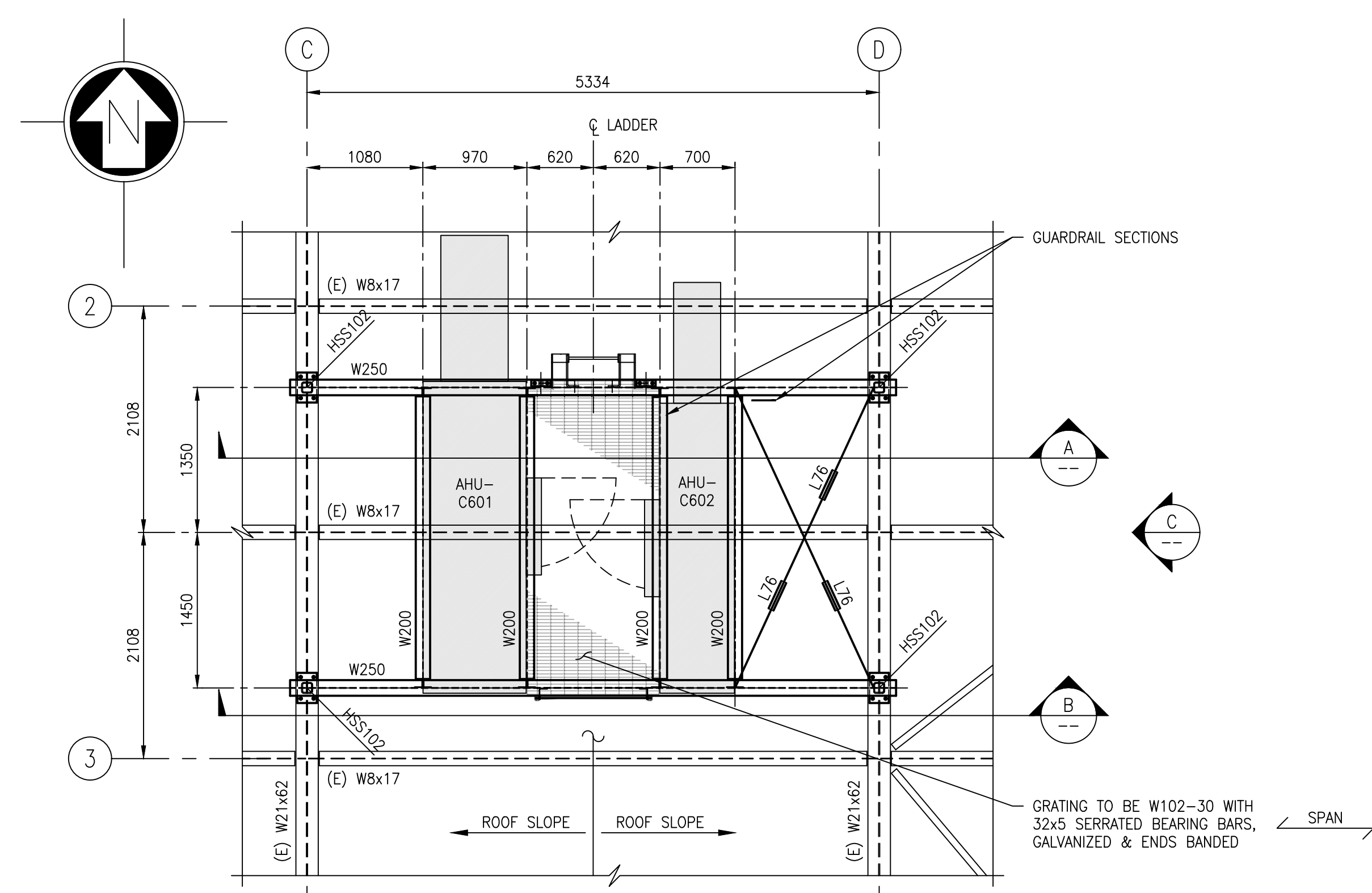
PLAN - PARTIAL ROOF SCALE: 1 : 40
