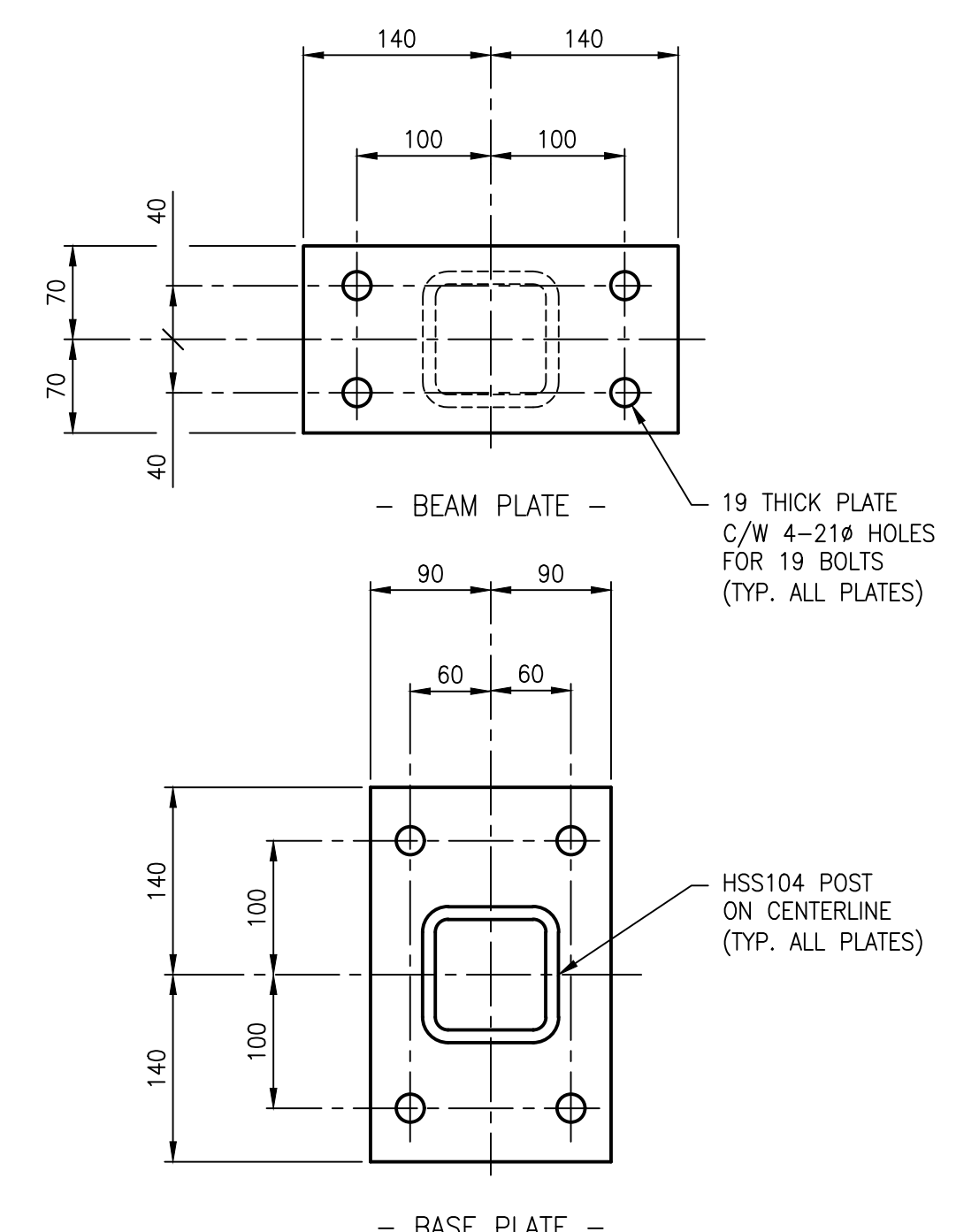
DETAIL - COLUMN PLATES SCALE: 1 : 5
