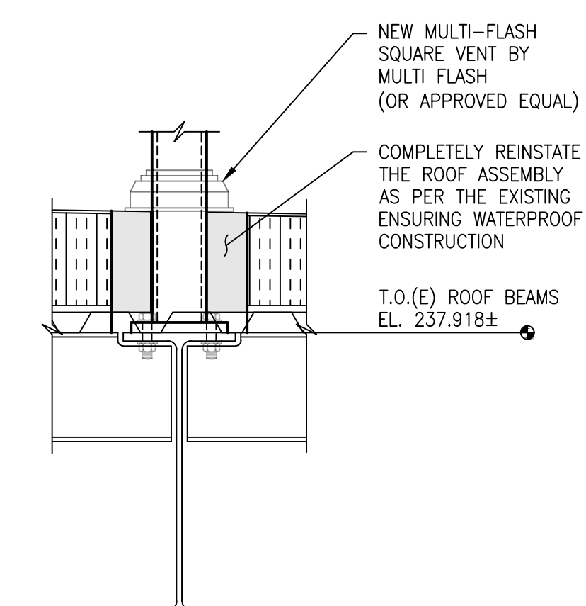
DETAIL - COLUMN FLASHING SCALE: 1 : 10
